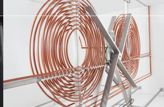
Double coil circular cooling system™ per fan tower zone
